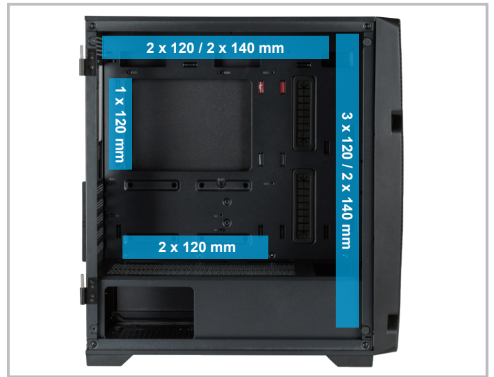
Maximum 8 Fans Installation
